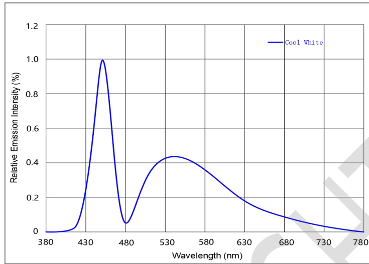
Fig.1-Spectrum Distribution
