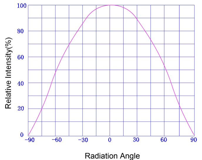
Fig.7- Directivity
