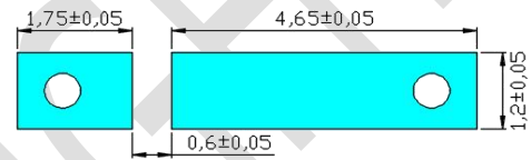
Recommended PCB solder PAD
