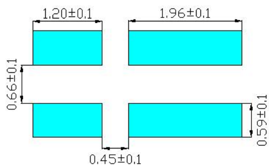
Recommended PCB solder PAD
