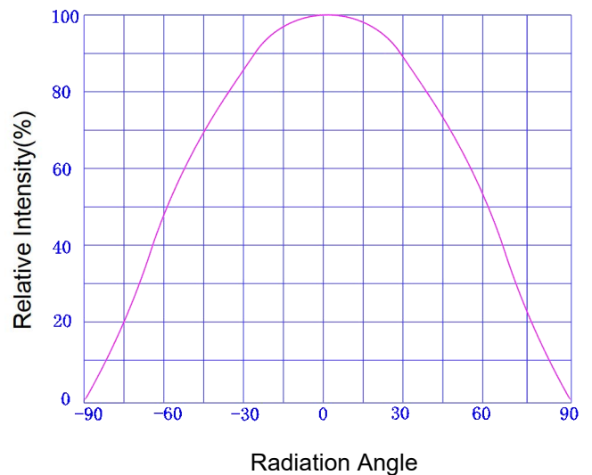
Fig.7- Directivity
